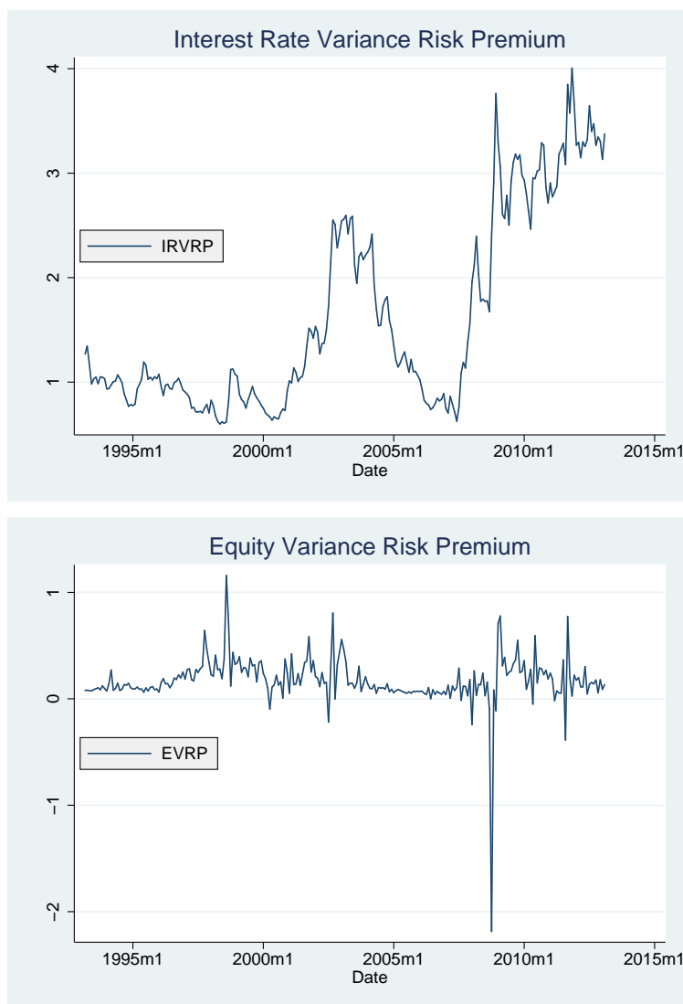
Figure 2: Time series of the interest rate and equity variance risk premium
